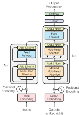
Figure: Vanilla transformer architecture
